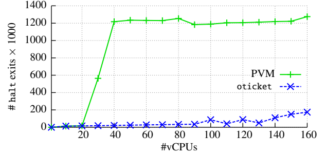
Figure 4: Number of halt exits that occur during a Linux kernel compile for two variants of spinlocks: in-stock ticket spinlock (PVM) and our oticket implementation.
