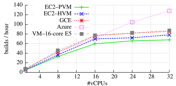
Figure 1: Performance of a Linux kernel compile on high-end VMs on Amazon EC2, Google Compute Engine, Microsoft Azure, and our in-house machine with similar hardware configuration. According to our experiment, cloud environments (except Azure) with increasing vCPU count do not guarantee scalable performance to end users.
