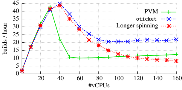
Figure 8: Performance impact of spinlock variants on Linux kernel compile for a single VM when co-scheduled with another exact VM instance running the same compilation.
