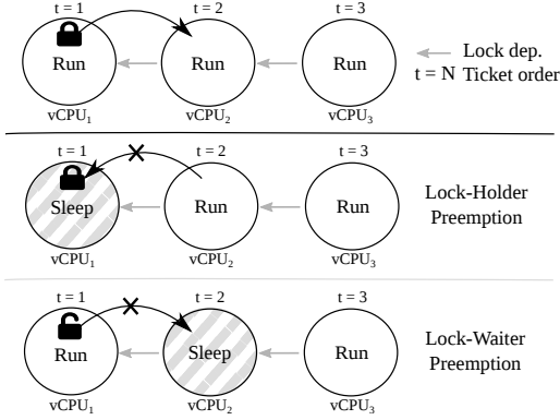
Figure 3: The issue of lock-holder preemption and lock-waiter preemption problem. Each of the circles represent a vCPU scheduled on a CPU. The Sleep state is the preempted vCPU whereas the Run state is the running one. t is the ticket order in which the vCPUs are waiting for the holder to release so that the waiters can acquire in FIFO order.
