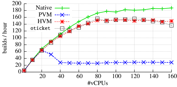
Figure 2: Performance of a Linux kernel compile on an 80-core machine. We enabled hyperthreads per core, similar to the cloud environments, and measured performance (builds/hour) on host (marked Native), PVM, HVM, and our own implementation, oticket. Unlike our speculation—hyperthreads being the only performance bottleneck as we observed from Figure 10— we found serious performance degradation in the PVM-based hypervisor at higher core counts.
