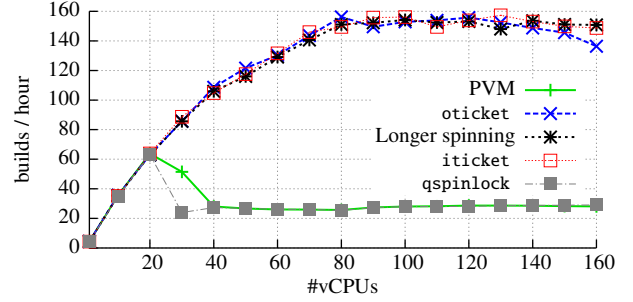
Figure 7: Linux kernel build performance for various FIFO based paravirtual spinlock implementations: Opportunistic ticket spinlock ( oticket ), ticket spinlock with longer spinning (Longer spinning), fine grained control of spinning period ( iticket ), and a MCS variant queue spinlock ( qspinlock ).
